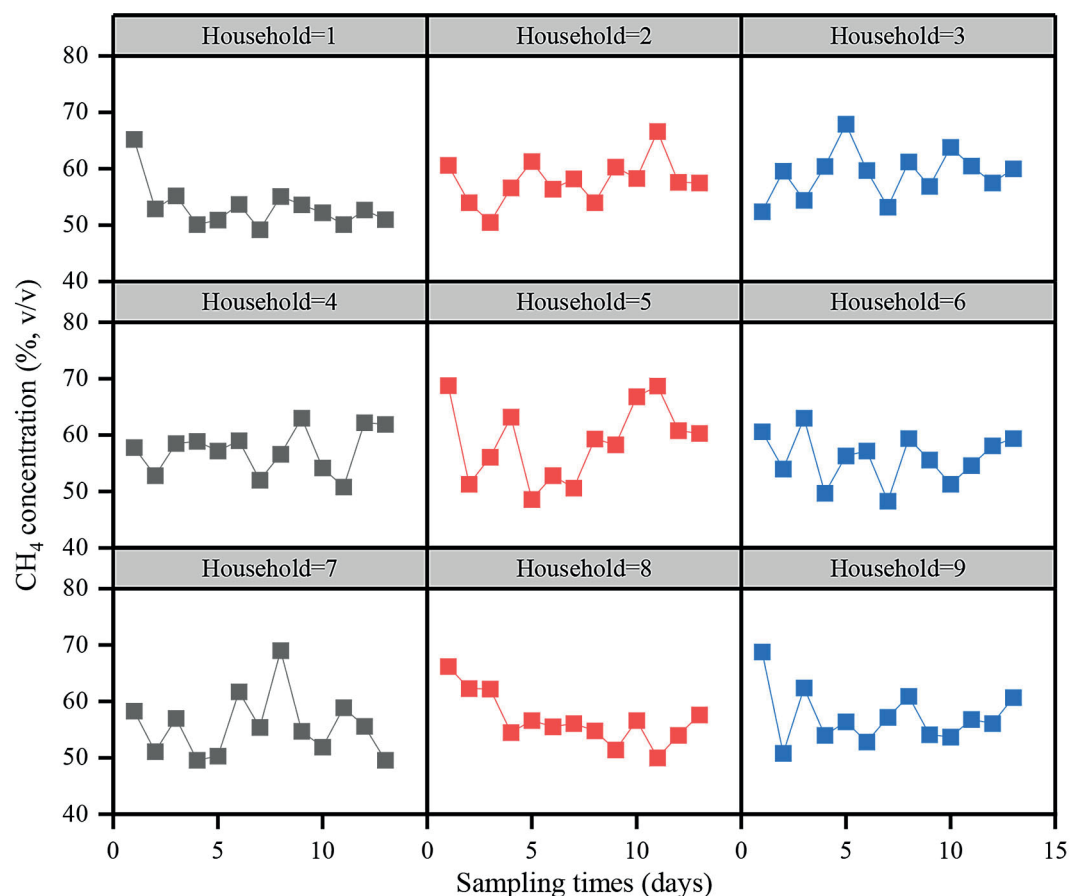
Figure 6. Methane concentration (% v/v) in biogas produced from each household-scale digester
