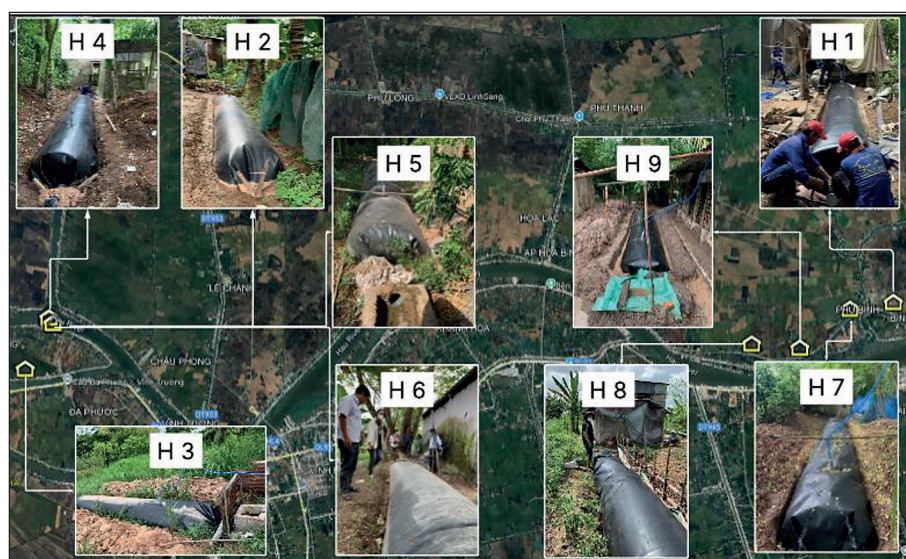
Figure 1. Installed sites of nine HDPE biogas digesters
