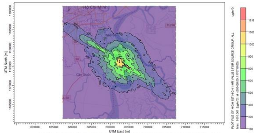
PLOT FILE OF HIGH 1ST HIGH 1-HR VALUES FOR SOURCE GROUP: ALL P1 (X: 677420.00 / Y: 1176210.00) - P2 (X: 707420.00 / Y: 1176210.00) - Step: 319.72 [m]
