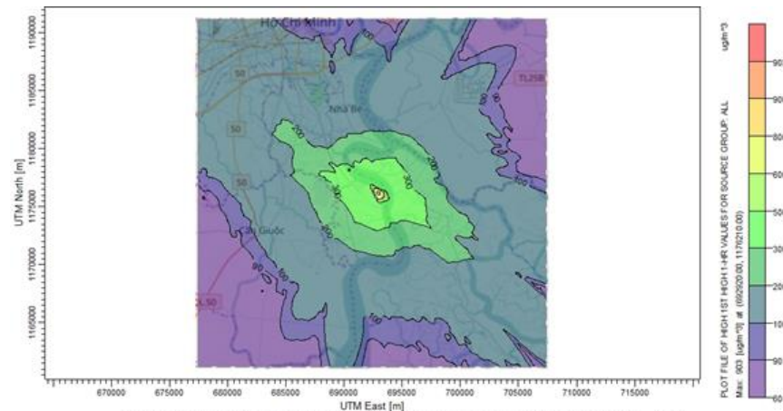
PLOT FILE OF HIGH 1ST HIGH 1-HR VALUES FOR SOURCE GROUP: ALL P1 (X: 677420.00 / Y: 1176210.00) - P2 (X: 707420.00 / Y: 1176210.00) - Step: 334.56 [m]
